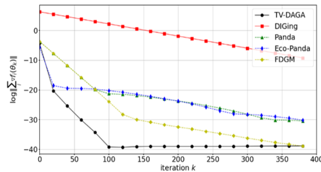
Fig. 3. Logistic classification problem on a network with n = 50 nodes and J = 200 data points per node, with data points being from the CIFAR-10 dataset.
