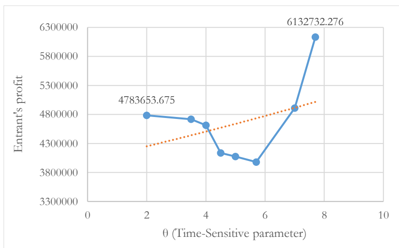
Fig. 4. Entrant's profit variations relative to time-sensitive parameter changes.
